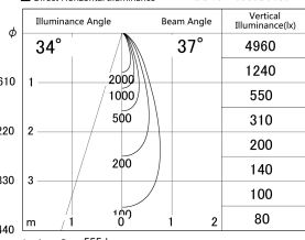
■ Direct Horizontal Illuminance DD161-0535B9035
