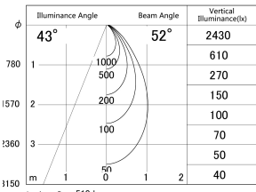
■ Direct Horizontal Illuminance DD161-0550B9035
