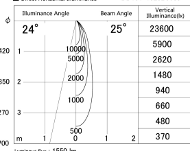
Direct Horizontal Illuminance DD161-1525B9035
