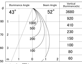
■ Direct Horizontal Illuminance DD161-0850B9040
