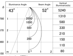
■ Direct Horizontal Illuminance DD161-1050B9040
