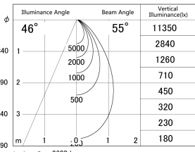
■ Direct Horizontal Illuminance DD161-2555B9040
