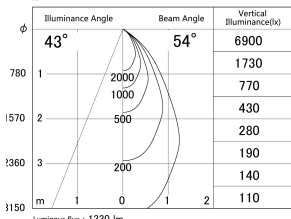
■ Direct Horizontal Illuminance DD140-1550MW9027D
