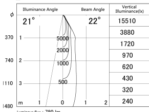
■ Direct Horizontal Illuminance DD140-0820MW9030D
