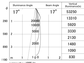
■ Direct Horizontal Illuminance DD140-2015MW9030D
