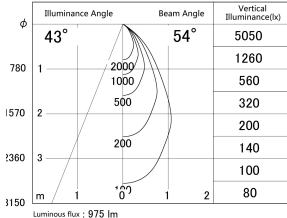
■ Direct Horizontal Illuminance DD140-1050MW9035D
