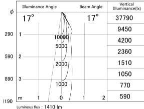
■ Direct Horizontal Illuminance DD140-1515MW9035D
