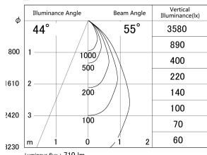
■ Direct Horizontal Illuminance DD140-0850MW9040D
