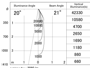
■ Direct Horizontal Illuminance DD140-2020MW9040D
