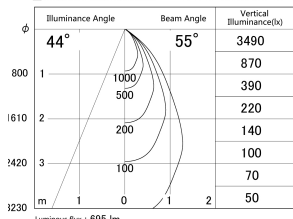
■ Direct Horizontal Illuminance DD140-0850MB9027D
