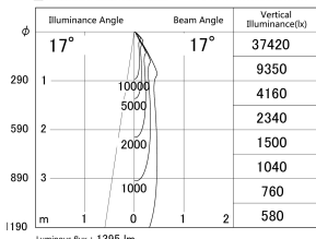
■ Direct Horizontal Illuminance DD140-1515MB9027D
