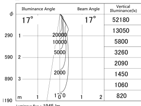
■ Direct Horizontal Illuminance DD140-2015MB9027D
