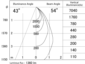
■ Direct Horizontal Illuminance DD140-1550MB9030D
