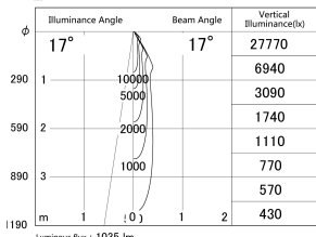
■ Direct Horizontal Illuminance DD140-1015MB9040D
