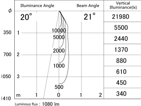
■ Direct Horizontal Illuminance DD140-1020MB9040D
