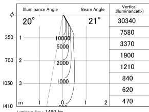
■ Direct Horizontal Illuminance DD140-1520MB9040D
