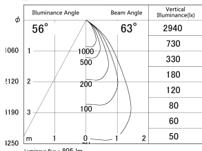
■ Direct Horizontal Illuminance DD140-1050DW9027D
