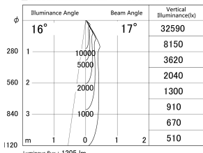
■ Direct Horizontal Illuminance DD140-1515DW9027D
