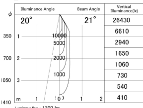
■ Direct Horizontal Illuminance DD140-1520DW9027D
