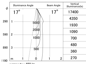
■ Direct Horizontal Illuminance DD140-0815DW9030D
