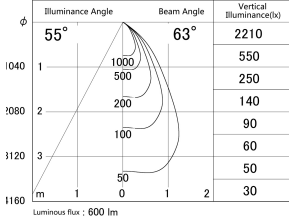
■ Direct Horizontal Illuminance DD140-0850DW9030D
