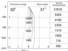
■ Direct Horizontal Illuminance DD140-2020DW9030D
