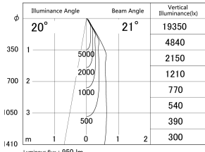
■ Direct Horizontal Illuminance DD140-1020DW9035D
