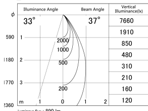
■ Direct Horizontal Illuminance DD140-1030DW9035D
