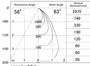
■ Direct Horizontal Illuminance DD140-1050DW9035D
