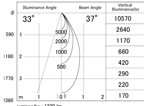
■ Direct Horizontal Illuminance DD140-1530DW9035D
