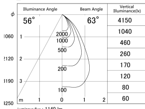
■ Direct Horizontal Illuminance DD140-1550DW9040D
