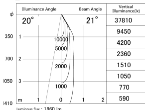
■ Direct Horizontal Illuminance DD140-2020DW9040D
