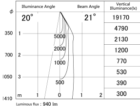
■ Direct Horizontal Illuminance DD140-1020DB9027D
