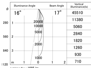
■ Direct Horizontal Illuminance DD140-2015DB9027D
