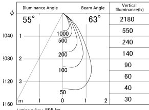
■ Direct Horizontal Illuminance DD140-0850DB9035D
