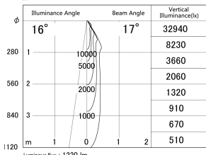
■ Direct Horizontal Illuminance DD140-1515DB9035D
