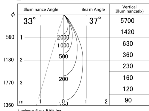
■ Direct Horizontal Illuminance DD140-0830DB9040D
