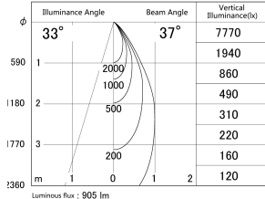
■ Direct Horizontal Illuminance DD140-1030DB9040D
