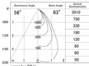
■ Direct Horizontal Illuminance DD140-1050DB9040D
