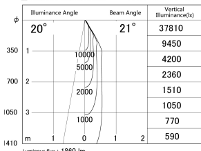
■ Direct Horizontal Illuminance DD140-2020DB9040D
