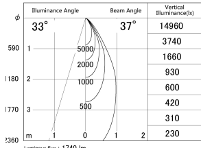
■ Direct Horizontal Illuminance DD140-2030DB9040D
