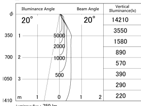
■ Direct Horizontal Illuminance DD140-0820WW9027D
