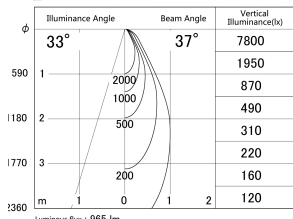
■ Direct Horizontal Illuminance DD140-1030WW9027D
