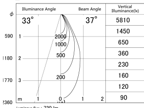
■ Direct Horizontal Illuminance DD140-0830WW9030D
