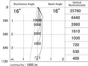
■ Direct Horizontal Illuminance DD140-1015WW9030D
