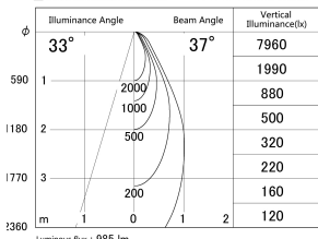
■ Direct Horizontal Illuminance DD140-1030WW9030D
