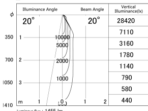
■ Direct Horizontal Illuminance DD140-1520WW9030D
