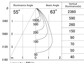
■ Direct Horizontal Illuminance DD140-0850WW9035D
