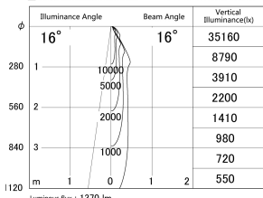
■ Direct Horizontal Illuminance DD140-1515WW9035D
