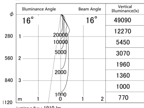
■ Direct Horizontal Illuminance DD140-2015WW9035D
